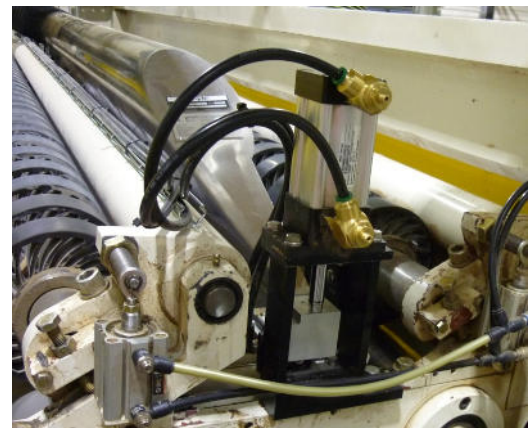
Individual design of the lower manifold considering the movement of the trim box.
