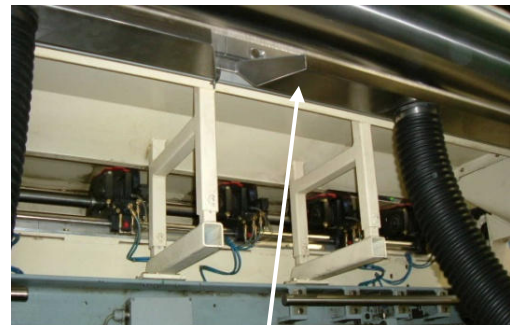
Individual design of the lower manifold considering the movement of the trim box.
